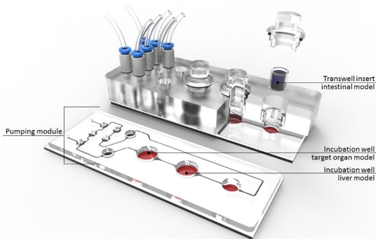
Fig. 2: Microfluidic platform for long-term multi-tissue coculture with closed circuit
